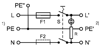
Figure 1: 2-pole version of a power entry module
